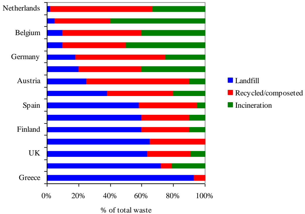
Figure 14. Landfill, recycled, composted and incineration in European countries.
