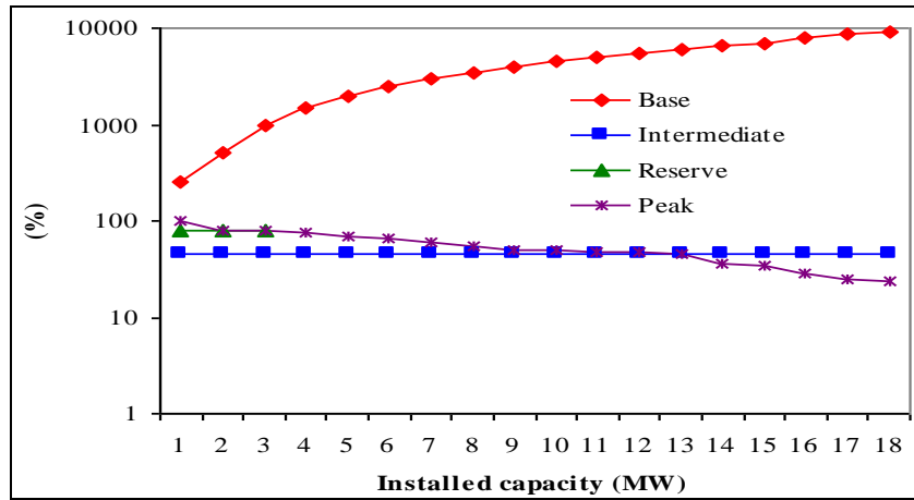
Figure 13. PV installed capacity (MW).
