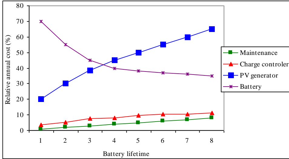
Figure 12. Battery lifetime versus relative annual cost (%).
