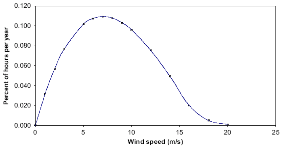
Figure 2. Yearly wind probability density ( k = 1.99 , c = 7.81\text{ms}^{-1} ).
