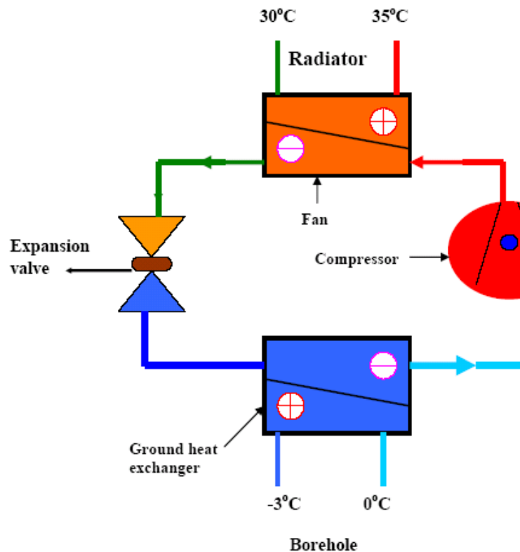
Figure 2. Detail of the GSHP circuit.
