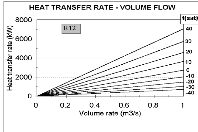
Figure 5. Heat transfer rate versus volume rate.
