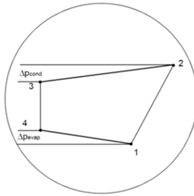
Figure 18. Pressure drops in evaporator and condenser.
