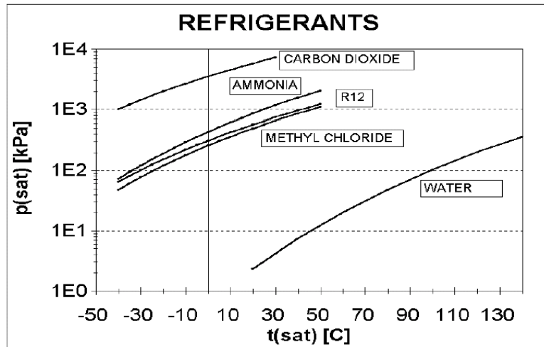
Figure 9. Refrigerant chart.
