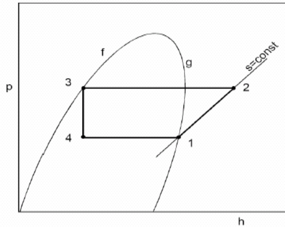
Figure 14. Refrigeration cycle.
