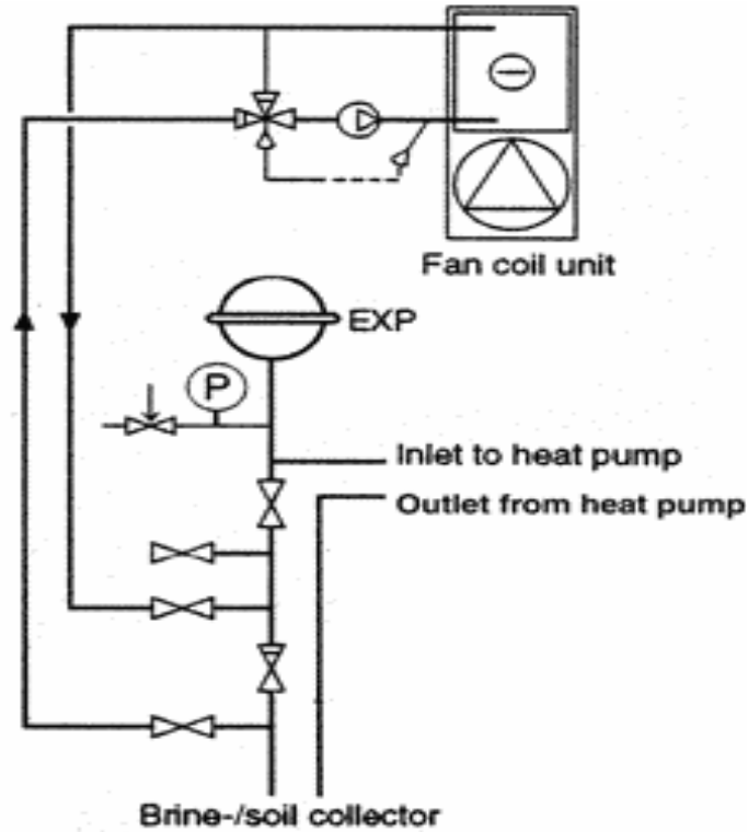
Figure 3. Diagram of cooling system.
