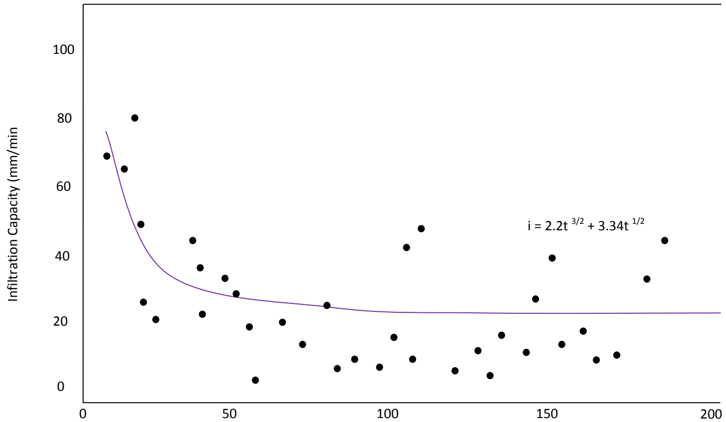
Fig. 3: Initial Infiltration Capacity Soil Moisture
